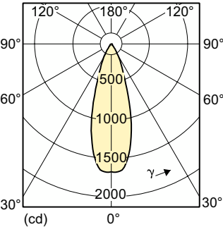
Light Distribution Diagram – 8.5MRX16/F35 2700 DIM AF 10/1
