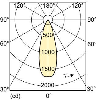
Light Distribution Diagram - MASTER LED 8-50W+ 830 MR16 36D Dim
