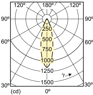
Light Distribution Diagram - MAS LEDspotLV VLE D6.3-35W 840MR16 36DRS
