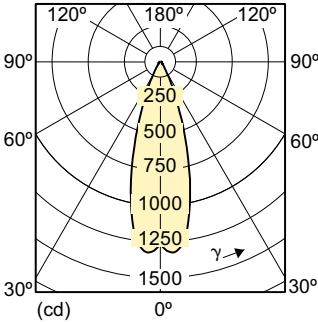
Light Distribution Diagram - MASTER LED 7-50W 930 MR16 36D Dim CN
