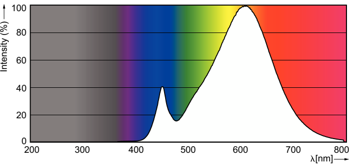
Spectral Power Distribution Colour - MAS LEDspotLV D 7-35W 827 MR16 60D
