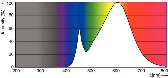
Spectral Power Distribution Colour - MASTER LED 7W 830 MR16 60D Dim AU
