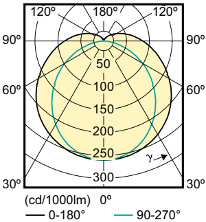
Light Distribution Diagram - MAS LEDtube 900mm 15W840 T8 RN
