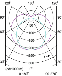
Light Distribution Diagram - 15T8/48-4000 IF 10/1 TAA
