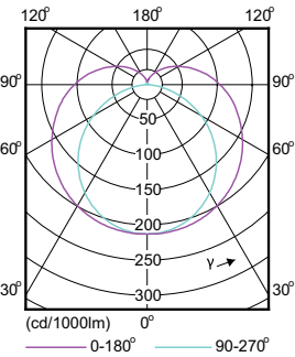
Light Distribution Diagram - 15T8/48-5000 IF 10/1
