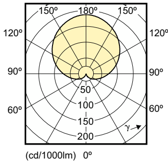
Light Distribution Diagram - CorePro LEDbulb 9.5-60W 830 E27
