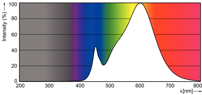
Spectral Power Distribution Colour - CorePro LEDbulb 9.5-60W 830 E27
