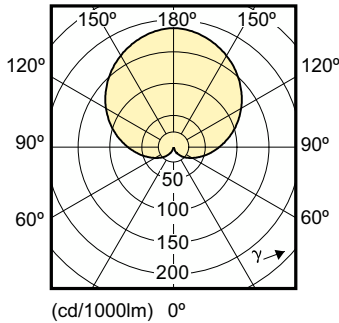
Light Distribution Diagram - LEDBulb 9.5-60W E27 3000K 230V A60 AU/PF
