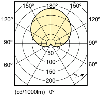
Light Distribution Diagram - LEDBulb 9.5-60W E27 3000K A60 3PK/6 AU
