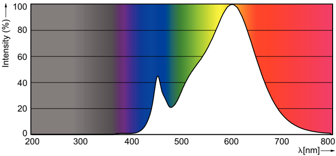
Spectral Power Distribution Colour - LEDBulb 9.5-70W E27 830 220-240V 3PF/10
