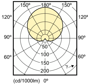
Light Distribution Diagram - LEDBulb 9.5-70W E27 830 220-240V 3PF/10
