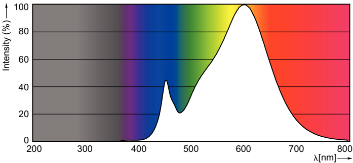
Spectral Power Distribution Colour - LEDBulb 10.5-75W B22 3000K 230V A60AU/PF
