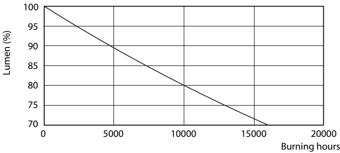
Lumen Maintenance Diagram - LEDBulb 10.5-75W E27 6500K 230V A60AU/PF
