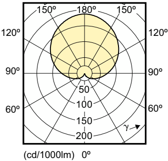
Light Distribution Diagram - LEDBulb 10.5-75W E27 6500K 230V A60AU/PF
