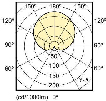
Light Distribution Diagram - LEDBulb 13-100W E27 865 220-240V 1PF/12
