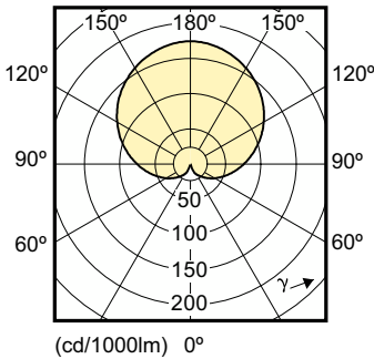
Light Distribution Diagram - LEDBulb 13-90W E27 6500K 230V A60 AU/PF
