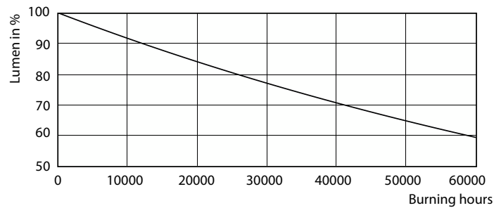
Lumen Maintenance Diagram - MAS LEDspotLV D 15-75W 927 AR111 24D
