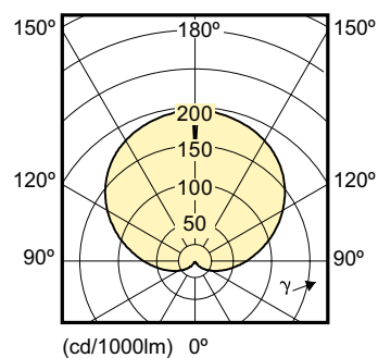
Light Distribution Diagram - CorePro LEDbulb 13.5-100W 827 E27
