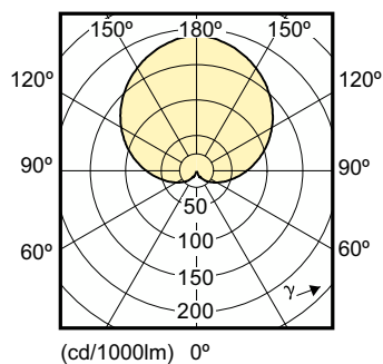
Light Distribution Diagram - CorePro LEDbulb 6-40W 827 B22
