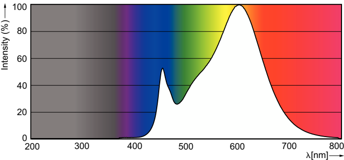
Spectral Power Distribution Colour - MAS LEDtube 1200mm 18W830 T8 I
