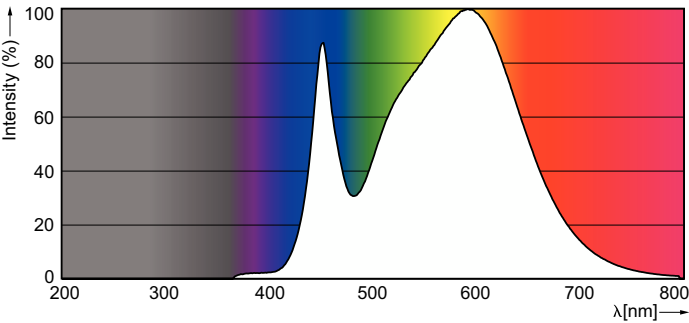
Spectral Power Distribution Colour - CorePro LEDbulb 13-100W 840 E27
