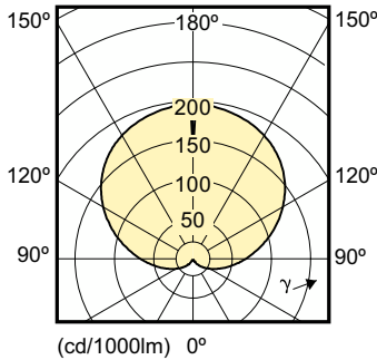
Light Distribution Diagram - CorePro LEDbulb 13-100W 840 E27
