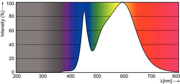
Spectral Power Distribution Colour - CorePro LEDbulb 10-75W 840 E27
