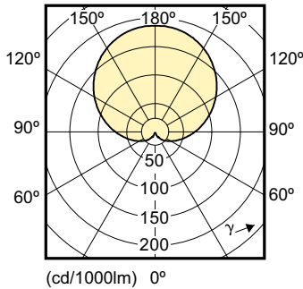
Light Distribution Diagram - CorePro LEDbulb 10-75W 840 E27
