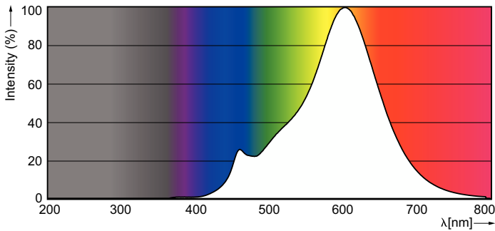
Spectral Power Distribution Colour - CLA LEDBulb ND 4.3-40W E27 WW A60 CL
