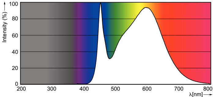
Spectral Power Distribution Colour - 8.5PL-C/T LED/26H-4000 IF 4P 10/1
