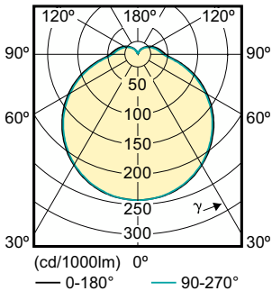
Light Distribution Diagram - 10.5PL-C/T LED/26V-4000 IF 4P 10/1
