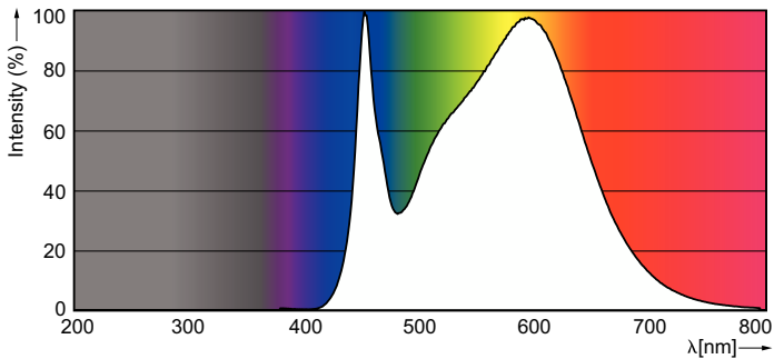
Spectral Power Distribution Colour - 10.5PL-C/T LED/26V-4000 IF 4P 10/1
