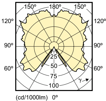
Light Distribution Diagram - 7A19/LED/827-22/CL/DIM 120V
