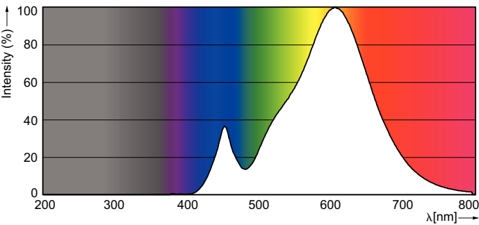
Spectral Power Distribution Colour - 10A19/LED/827-22/CL/DIM 120V
