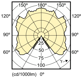
Light Distribution Diagram - 10A19/LED/827-22/CL/DIM 120V
