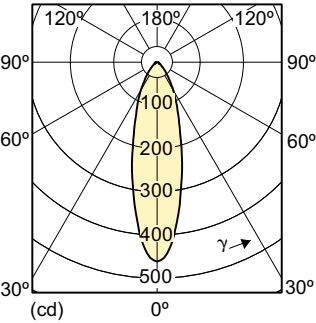
Light Distribution Diagram - CLA LEDspotLV ND 3-20W MR16 827 36D
