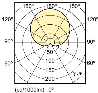
Light Distribution Diagram - LEDBulb 9-60W E27 3000K W A19 2PK/4
