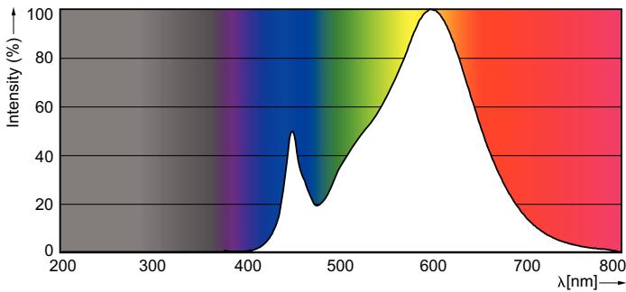
Spectral Power Distribution Colour - LEDBulb 9-60W E27 3000K W A19 2PK/4
