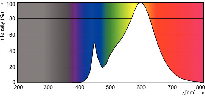
Spectral Power Distribution Colour - LEDBulb13.5W E27 3000K W A67 1BL/6 BR
