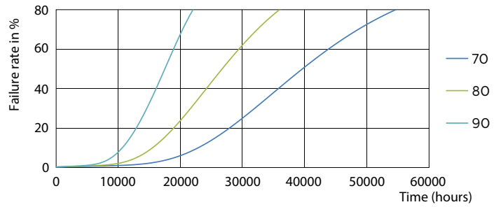
Life Expectancy Diagram - LED PLC 8.5W 830 2P G24d-3
