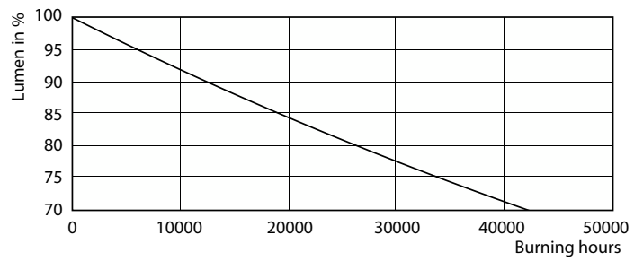
Lumen Maintenance Diagram - LED PLC 8.5W 830 2P G24d-3
