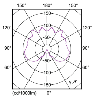
Light Distribution Diagram - 5.5A15/LED/827-22/E12/CL/DIM 120V
