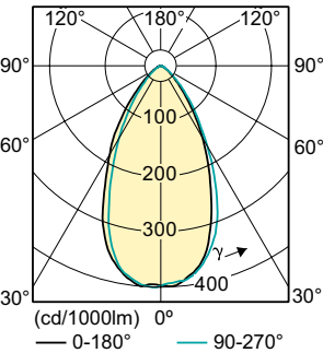
Light Distribution Diagram - MAS LEDspotMV VLE D 4.3-50W GU10 830 60D
