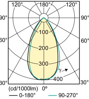
Light Distribution Diagram - MAS LEDspotMV VLE D 4.3-50W GU10 840 60D
