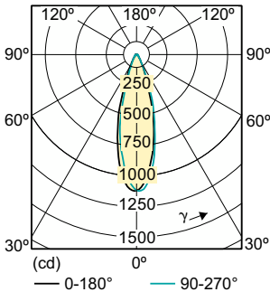
Light Distribution Diagram - CorePro LEDspotMV 5-50W GU10 827 36D
