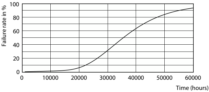
Life Expectancy Diagram - CorePro LEDspotMV 5-50W GU10 827 36D
