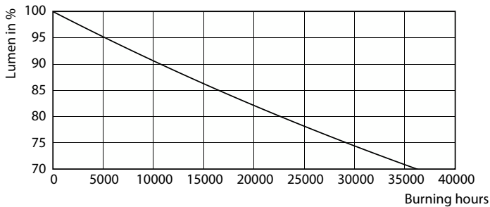
Lumen Maintenance Diagram - CorePro LEDspotMV 5-50W GU10 827 36D
