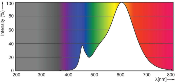
Spectral Power Distribution Colour - CorePro LEDspotMV 5-50W GU10 827 36D
