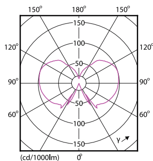
Light Distribution Diagram - CLA LEDLuster D 3-25W P45 E14 827 CL
