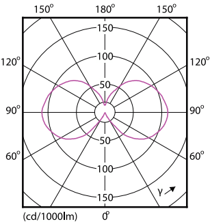
Light Distribution Diagram - CLA LEDLuster D 4.5-40W P45 E14 827 CL
