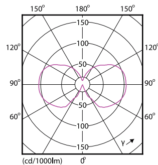
Light Distribution Diagram - CLA LEDBulb D 4.5-40W A60 E27 827 CL
