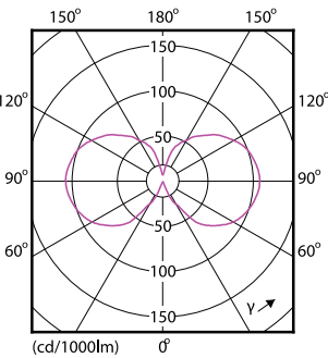
Light Distribution Diagram - CLA LEDGlobe D 7-60W G93 E27 827 CL
