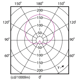
Light Distribution Diagram - CorePro LEDbulb D 6-40W A60 E27 827
