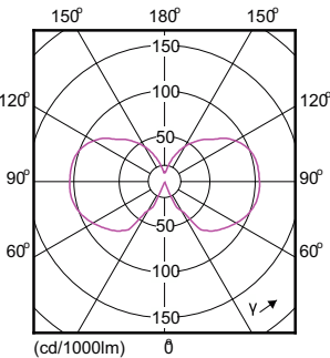
Light Distribution Diagram - CLA LEDBulb ND 4-40W A60 E27 827 CL
