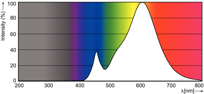
Spectral Power Distribution Colour - CLA LEDBulb ND 6-60W A60 E27 827 CL
