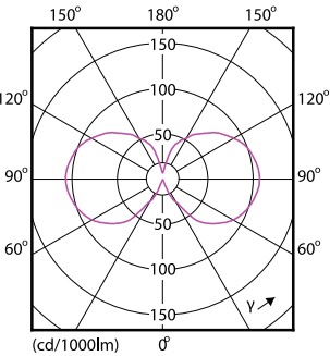
Light Distribution Diagram - CLA LEDBulb ND 6-60W A60 E27 827 CL
