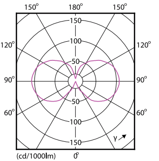
Light Distribution Diagram - CLA LEDBulb ND 6-60W A60 E27 827 CL
