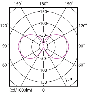
Light Distribution Diagram - CLA LEDBulb ND 6-60W ST64 E27 827 CL
