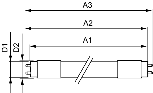
TLED 2ft 220-240V 9W-18W 3000K G13 ND
