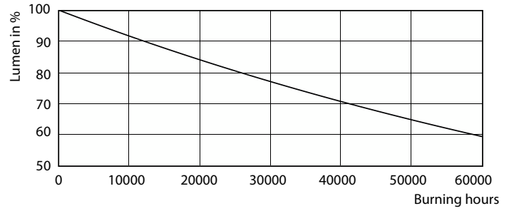
Lumen Maintenance Diagram - 12AR111/LED/930/S8 DIM 12V FB 1PK 6/1
