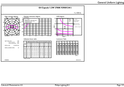
General uniform lighting - CorePro LEDcapsuleLV 1.2-10W G4 827
