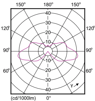
Light Distribution Diagram - CorePro LEDcapsuleLV 1.2-10W G4 827
