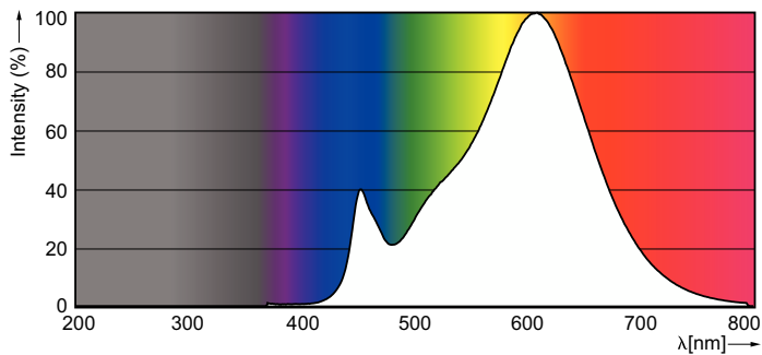
Spectral Power Distribution Colour - LED 4.5W 500mm S14D WW ND 1CT/4
