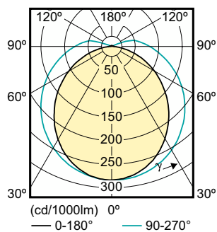
Light Distribution Diagram - LED 4.5W 500mm S14D WW ND 1CT/4
