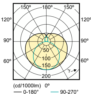
Light Distribution Diagram - CorePro LEDtube HF 1500mm 20W865 T8 G
